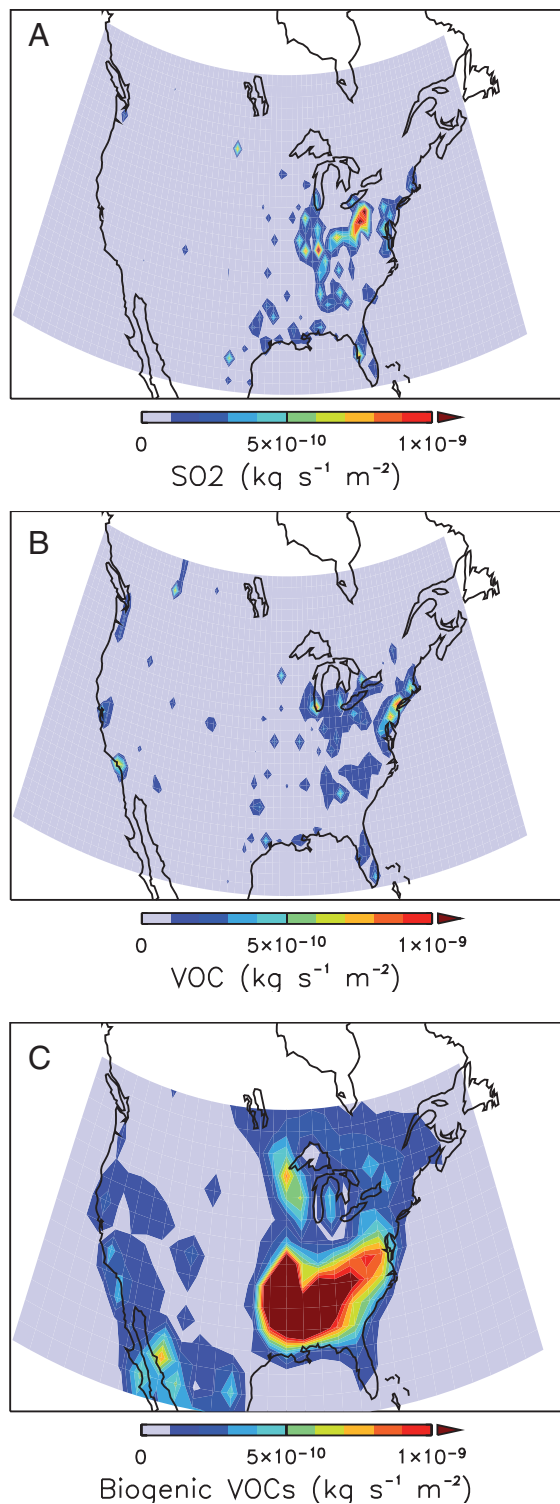
Fig. 2. Emission maps for the United States. (A) Annual total anthropogenic \text{SO}_2 emission. (B) Annual anthropogenic VOC emissions. (C) Annual total biogenic emissions of isoprene and monoterpenes. Anthropogenic Emissions are from U.S. Environmental Protection Agency National Emissions Inventory version 3 (NEI-99) (18), regridded from 4 km to 1^\circ resolution.
