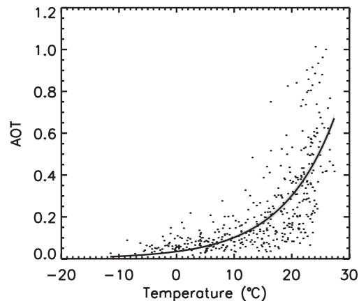
Fig. 3. Comparison of Walker Branch AERONET AOT (440 nm) vs. corresponding NCEP SE mean surface temperature reconstructions. Curve is exponential following the temperature dependence of biogenic VOC emission (28): \gamma = \exp[\beta(T - T_s)] , where \beta is an empirical coefficient of exponential dependence and T_s is the base temperature of standard conditions (303 K). The best-fit curve shown above ( R^2 = 0.55 ) has a \beta of 0.11, in good agreement with BVOC emission observations.
