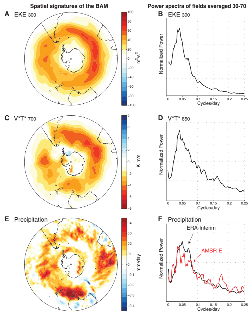
Fig. 1. (A to F) Space and time signatures of the Southern Hemisphere BAM. The left panels show the fields indicated regressed onto the BAM index time series (12, 13, 15). The right panels show power spectra for hemispheric averages of the fields indicated (17). Red values in (C) denote southward (negative) heat fluxes. The spectra in (F) show results for precipitation derived from ERA-Interim [black (11)] and AMSR-E [red (11)]. All other panels are based on the ERA-Interim model (11). As discussed in the text, the heat fluxes and precipitation peak 1 day before the peak in eddy-kinetic energy, and thus the regressions in (C) and (E) are lagged by -1 day with respect to the BAM index.
