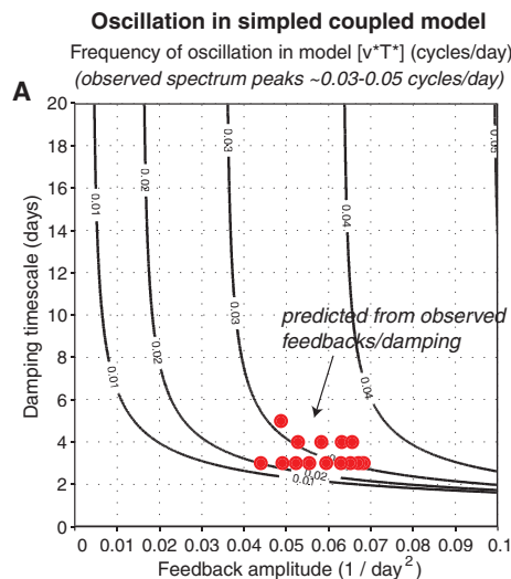
Fig. 3. Simulating periodic behavior in the heat fluxes in a simple coupled model. (A) The analytic solution of the oscillation frequency in the eddy fluxes of heat obtained from the simple model of Eqs. 2 and 3. Results are shown as a function of the product of the model feedback parameters ( \alpha \times \beta ; abscissa) and damping time scale (ordinate). Frequency units are cycles per day. Red circles indicate the range of frequencies predicted from the observed feedbacks and damping time scales at all tropospheric levels. (B) Power spectra derived from the simple model using the feedback parameters at 500 hPa for the damping time scales indicated. The observed spectrum is for Southern Hemisphere mean eddy kinetic energy and is reproduced from Fig. 1B. See the supplementary materials for details of the calculations.
