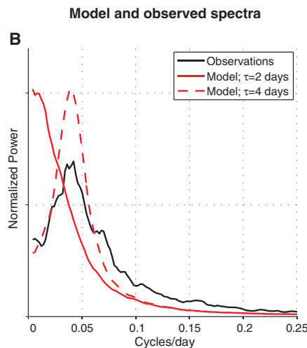
Fig. 3. Simulating periodic behavior in the heat fluxes in a simple coupled model. (A) The analytic solution of the oscillation frequency in the eddy fluxes of heat obtained from the simple model of Eqs. 2 and 3. Results are shown as a function of the product of the model feedback parameters ( \alpha \times \beta ; abscissa) and damping time scale (ordinate). Frequency units are cycles per day. Red circles indicate the range of frequencies predicted from the observed feedbacks and damping time scales at all tropospheric levels. (B) Power spectra derived from the simple model using the feedback parameters at 500 hPa for the damping time scales indicated. The observed spectrum is for Southern Hemisphere mean eddy kinetic energy and is reproduced from Fig. 1B. See the supplementary materials for details of the calculations.
