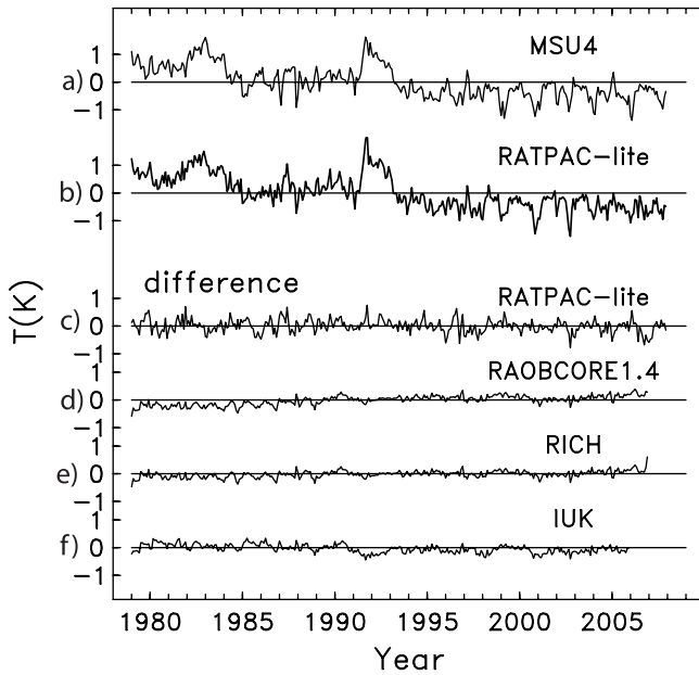
Figure 7. Time series of (a) deseasonalized zonal mean UAH MSU4 anomalies and (b) vertically-integrated RATPAC-lite radiosonde anomalies for data averaged over 60^{\circ}\text{N} – ^{\circ}\text{S} . (c, d, e, f) (MSU4 minus radiosonde) differences for four radiosonde data sets, as indicated.
