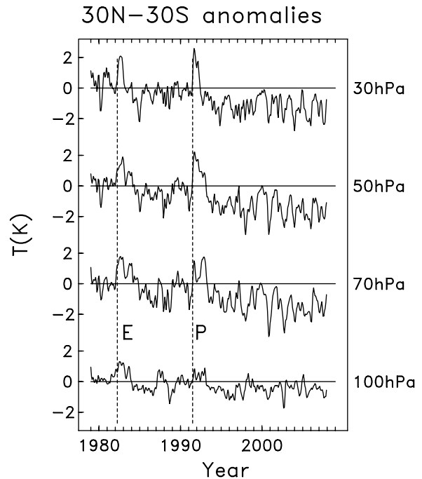
Figure 10. Time series of tropical ( 30^{\circ}\text{N} – 30^{\circ}\text{S} ) lower stratosphere temperature anomalies at individual pressure levels derived from RATPAC-lite data. E and P denote the volcanic eruptions of El Chichon and Pinatubo, respectively.
