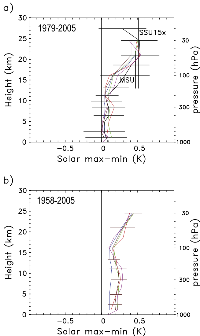
Figure 24. The vertical profile of the temperature solar signal in the tropics ( 30^{\circ}\text{N} – ^{\circ}\text{S} ) derived from the different radiosonde data for (a) 1979–2005 and (b) 1958–2005. Results are expressed as approximate differences between solar maximum and solar minimum, and error bars denote two-sigma statistical uncertainty estimates at each level. The colors denote the different radiosonde data sets with the same colors as Figure 23. The vertical bars in Figure 24a denote the corresponding satellite data results from UAH MSU4 data (for 1979–2007) and SSU15x (1979–2005).
