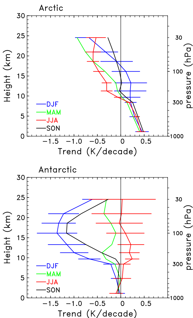
Figure 12. Vertical profile of polar temperature trends for 1979–2007, derived from RICH data, for the Arctic (top, 60^{\circ} – 90^{\circ} N) and Antarctic (bottom, 60^{\circ} – 90^{\circ} S). Results are shown on the basis of data for each season (December, January, and February (DJF), etc.). One-sigma uncertainty estimates are shown for the DJF and JJA results in each panel, and uncertainties for other seasons are similar.
