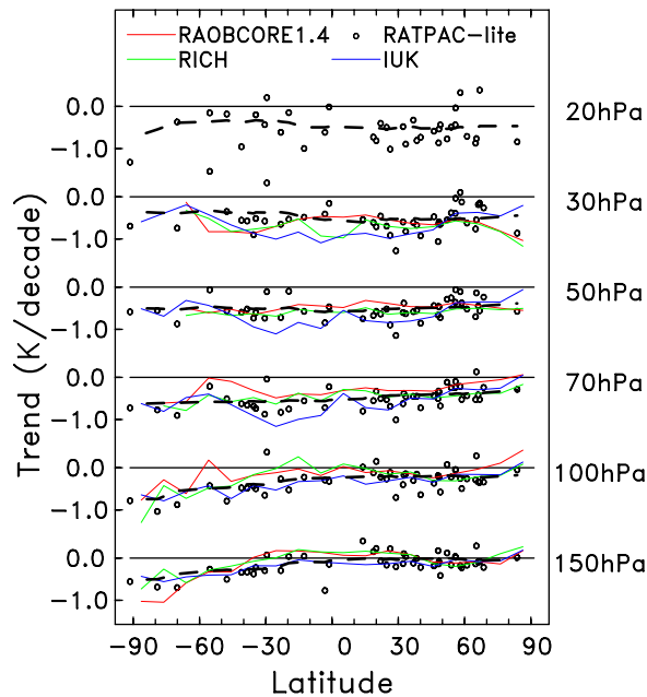
Figure 8. Latitudinal profile of annual mean temperature trends for 1979–2007 at pressure levels spanning 150–20 hPa, derived from each of the radiosonde data sets, as indicated. For each level, circles denote the trends at each of the individual RATPAC-lite stations, and the heavy dashed lines show a smooth latitudinal fit to the individual station trends.
