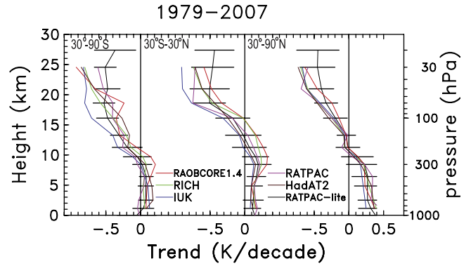
Figure 9. Vertical profile of annual mean temperature trends for 1979–2007 derived from the separate radiosonde data sets for latitude bands 30^{\circ} – 90^{\circ}\text{S} , 30^{\circ}\text{N} – ^{\circ}\text{S} , and 30^{\circ} – 90^{\circ}\text{N} . Error bars show the two-sigma statistical uncertainty levels for the RATPAC-lite data.
