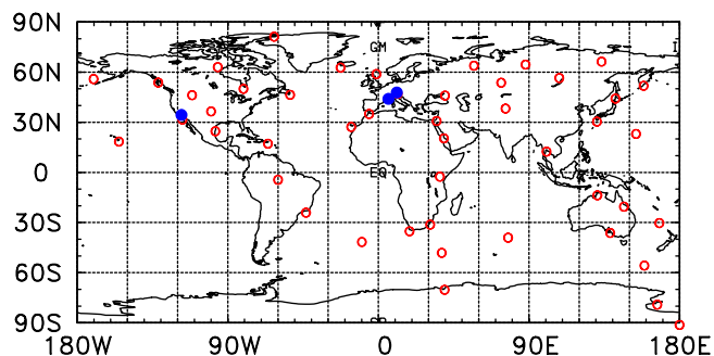
Figure 3. Locations of radiosonde stations for the RATPAC-lite data set (red circles) and lidar stations (blue dots) stations used here.
