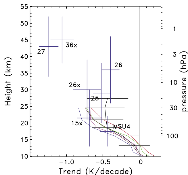
Figure 19. Vertical profile of temperature trends for 1979–2005 derived from each of the individual SSU and UAH MSU4 satellite data sets, averaged over 60^\circ\text{N} – ^\circ\text{S} . Vertical bars denote the approximate altitude covered by each channel, and horizontal bars denote two-sigma statistical trend uncertainties. Results are also shown for trends derived from radiosonde data averaged over 60^\circ\text{N} – ^\circ\text{S} . Color scale is the same as in Figure 9.
