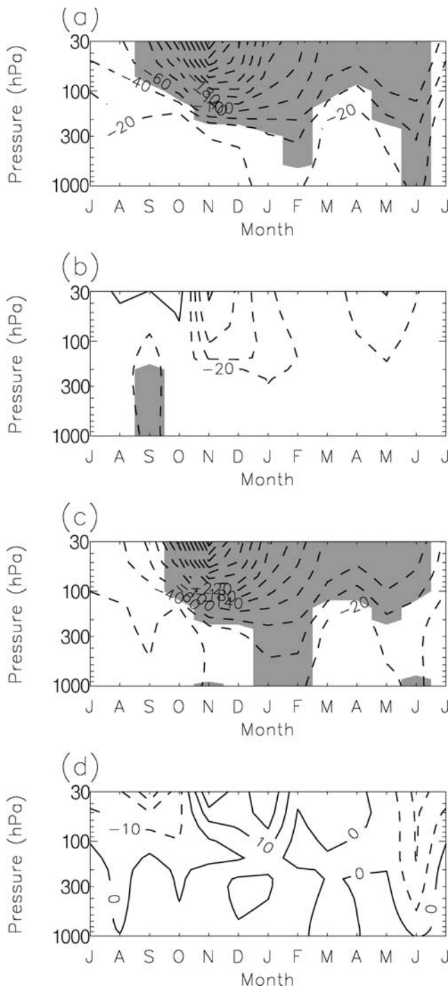
Figure 2. Average monthly mean geopotential height response (m) for the region south of 65°S. Anomalies relative to the control simulation are shown for the (a) full, (b) lower, and (c) midstratospheric ozone depletion experiments. (d) The difference between simulated geopotential height in the full and midstratospheric depletion experiments. Shading indicates regions of significance at the 95% level based on a two-sample t-test.
