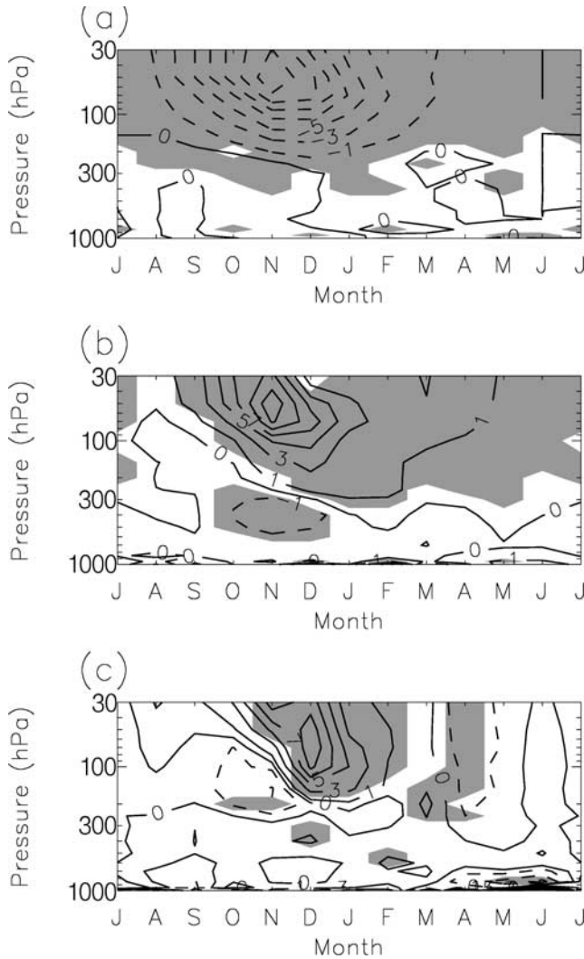
Figure 4. Heating components of the full ozone change (shown in Figure 1a) for (a) shortwave, (b) longwave, and (c) dynamical heating. Contour interval 2 \text{ K month}^{-1} (zero contour marked as well). Shading indicates regions of significance at the 95% level based on a two-sample t-test.
