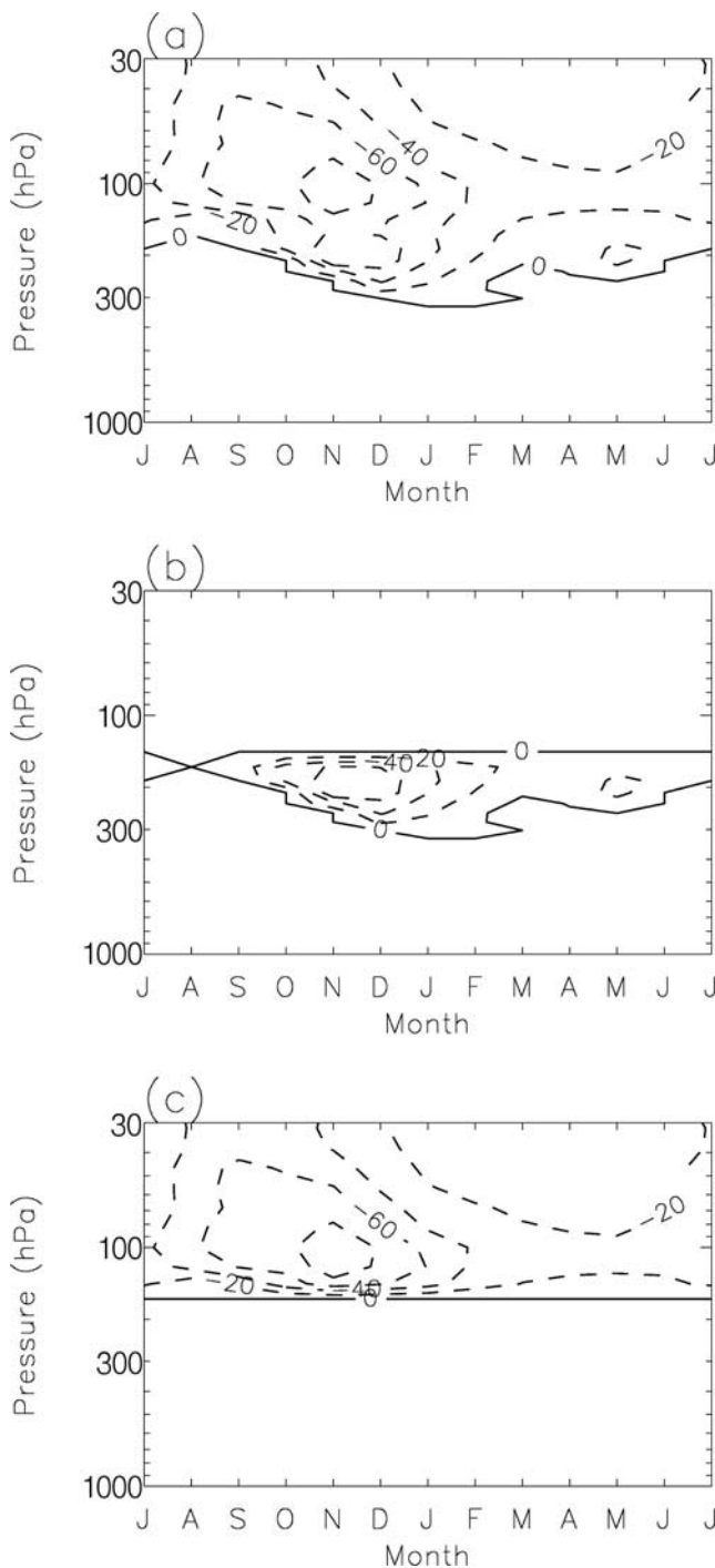
Figure 1. Percentage change in ozone for each month and pressure level at 70°S for (a) the whole stratosphere, (b) the lowermost stratosphere below 164 hPa (the ozone concentration in the troposphere remains constant so the zero contour marks the climatological tropopause in Figure 1a), and (c) the midstratosphere, above 164 hPa. The ozone changes shown in Figure 1a are identical to those used by GT03.
