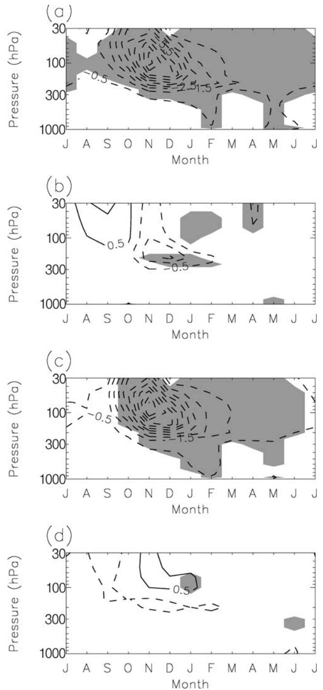
Figure 3. As Figure 2, except for the temperature response (K). The contour level separation is 1 K.
